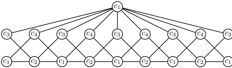
FIGURE 2. Equitable coloring of \check{P}_9
