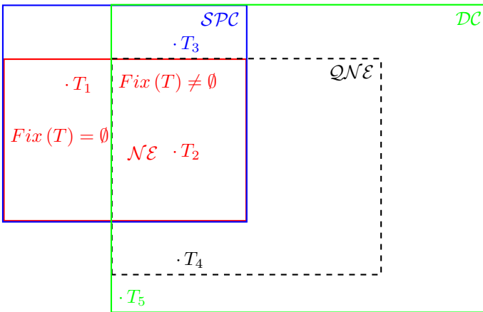
Figure 1. Diagram of the relationships between the classes \mathcal{NE} , \mathcal{QNE} , \mathcal{SPC} and \mathcal{DC}
